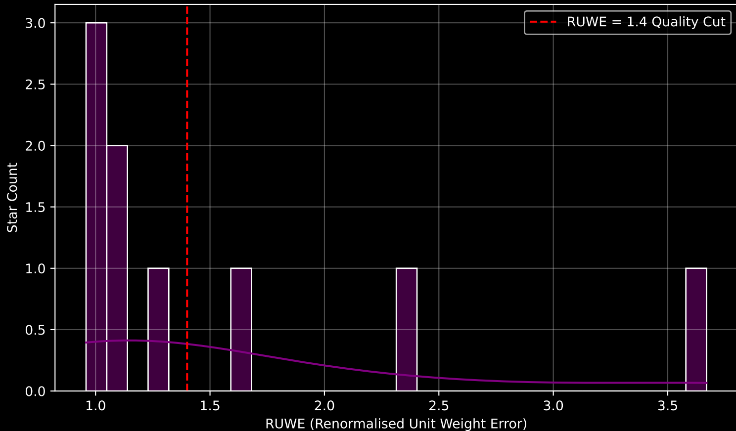
GALAH DR4 Field [7375] RUWE Distribution (n= 9)
