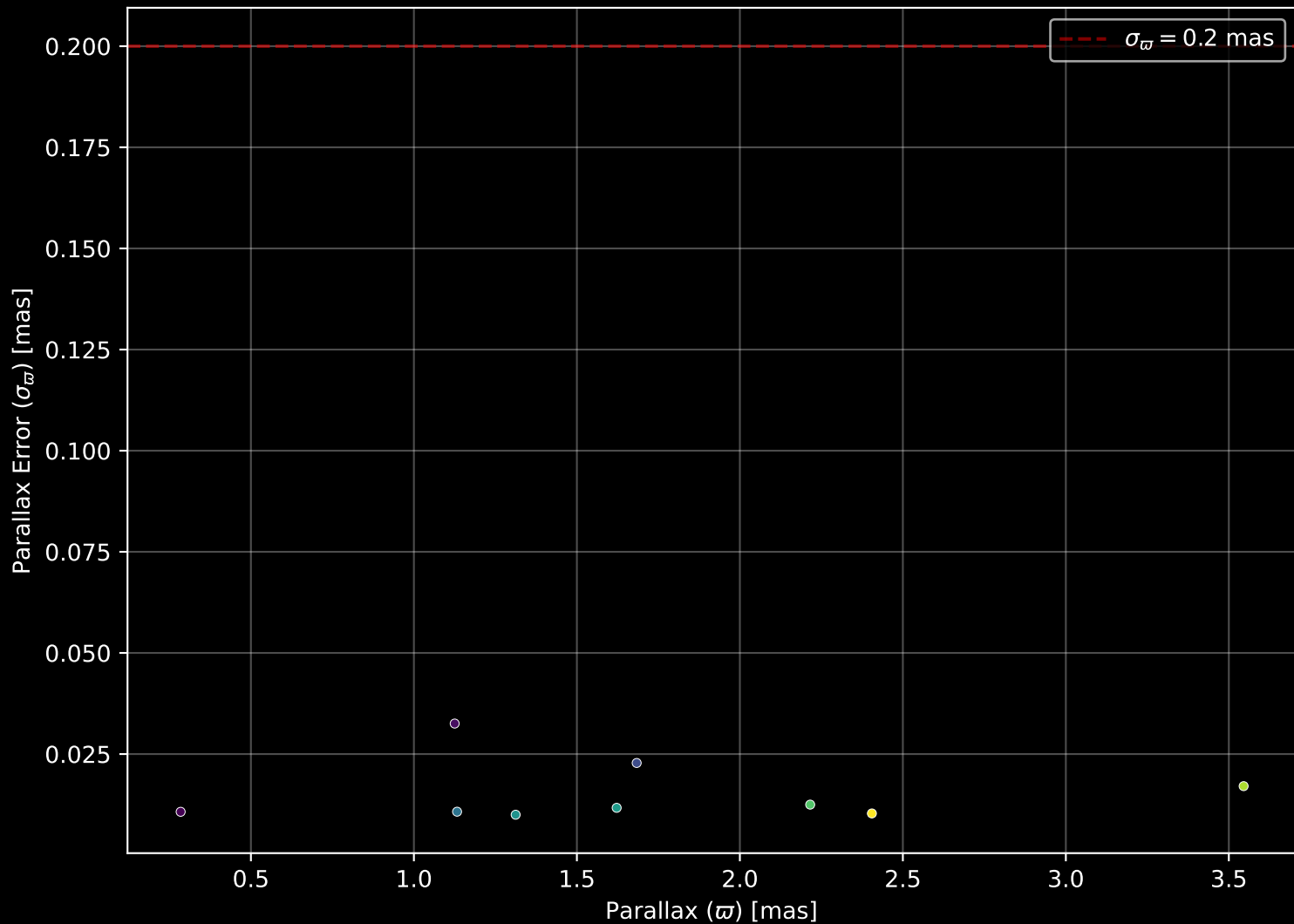
GALAH DR4 Field: [7375] Parallax Quality (n= 9)
