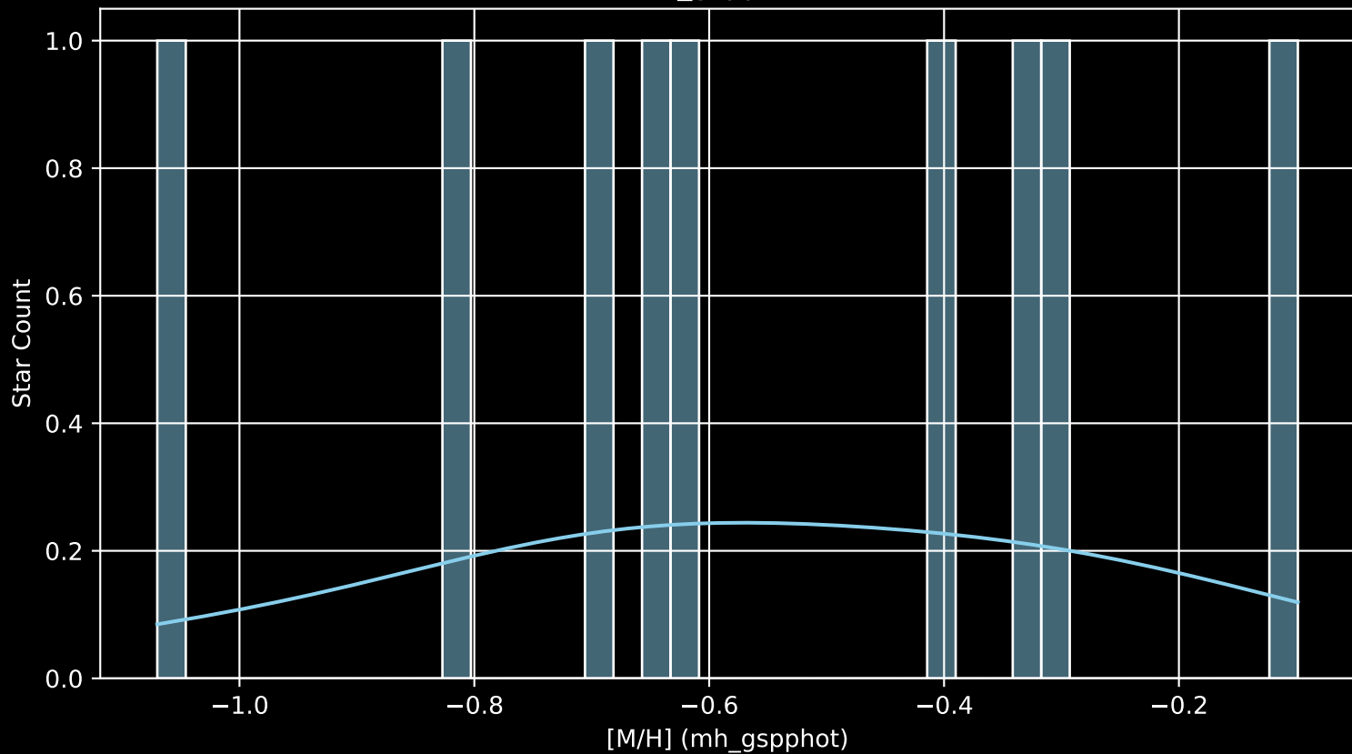
GALAH DR4 Field: [7375] [M/H] (mh_gspphot) (n= 9)
