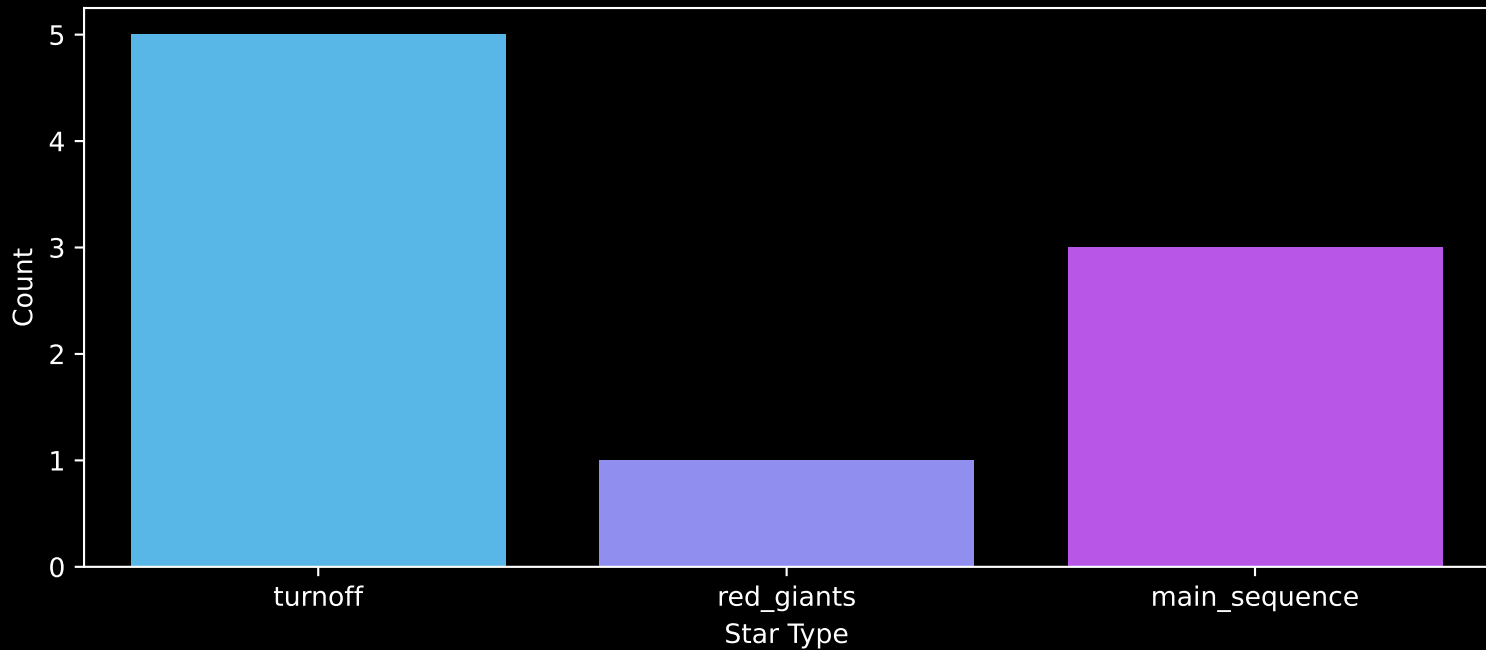
GALAH DR4 Field: [7375] Count plot of Star Type
