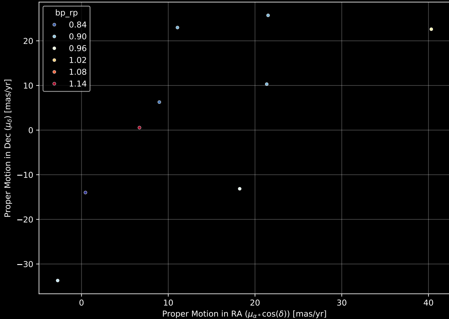
GALAH DR4 Field: [7375] Proper Motion Diagram (n= 9)
